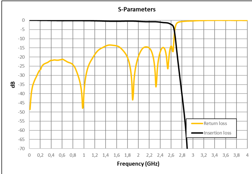
Figure 1:ERZ-LPF-0000-0250-1.3Insertion & Return loss
