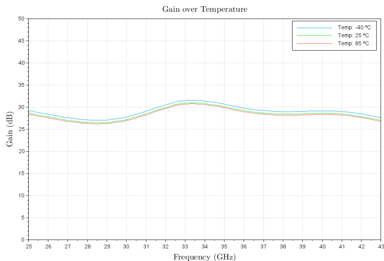
Figure 2: ERZ-LNA-2500-4300-33-2-NS Small Signal Gain
