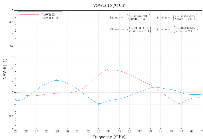
Figure 3: ERZ-LNA-2500-4300-33-2-NS Input&Output Matching
