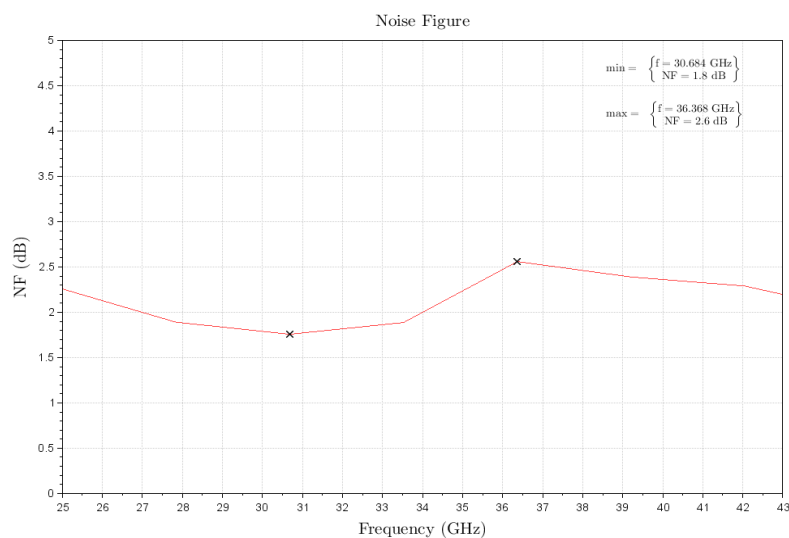
Figure 4: ERZ-LNA-2500-4300-33-2-NS Noise Figure
