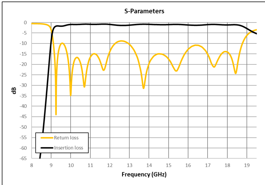
Figure 1: ERZ-HPF-0930-1870-1.7 Insertion & Return loss
