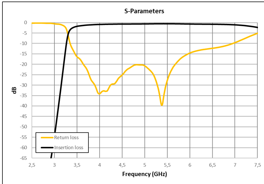
Figure 1:ERZ-HPF-0350-0690-1.7 Insertion & Return loss
