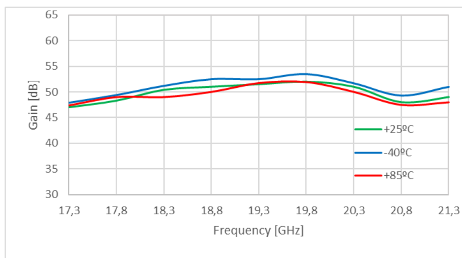
Figure 2: ERZ-HPA-1730-2120-44 Small Signal Gain
