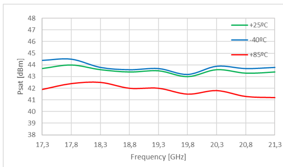
Figure 1: ERZ-HPA-1730-2120-44 Psat
