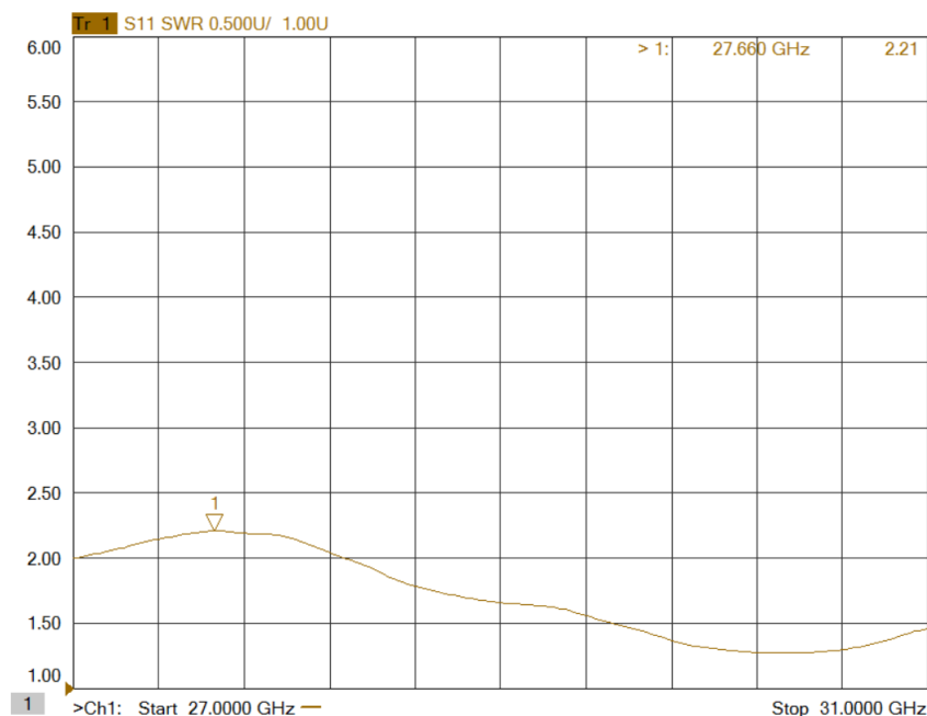
Figure 3: ERZ-HPA-1730-2120-44 Input Matching
