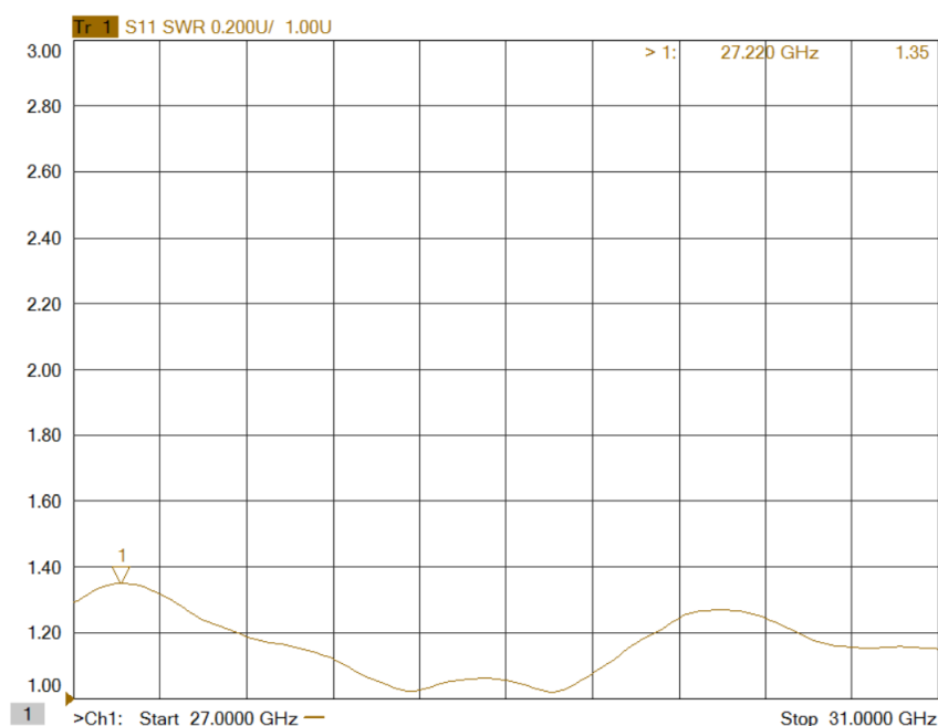
Figure 4: ERZ-HPA-1730-2120-44 Output Matching
