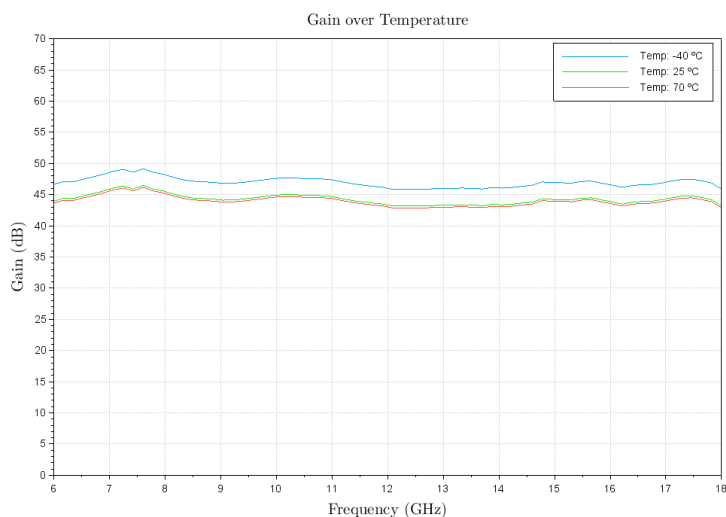
Figure 2: ERZ-HPA-0600-1800-40-E-NS Small Signal Gain
