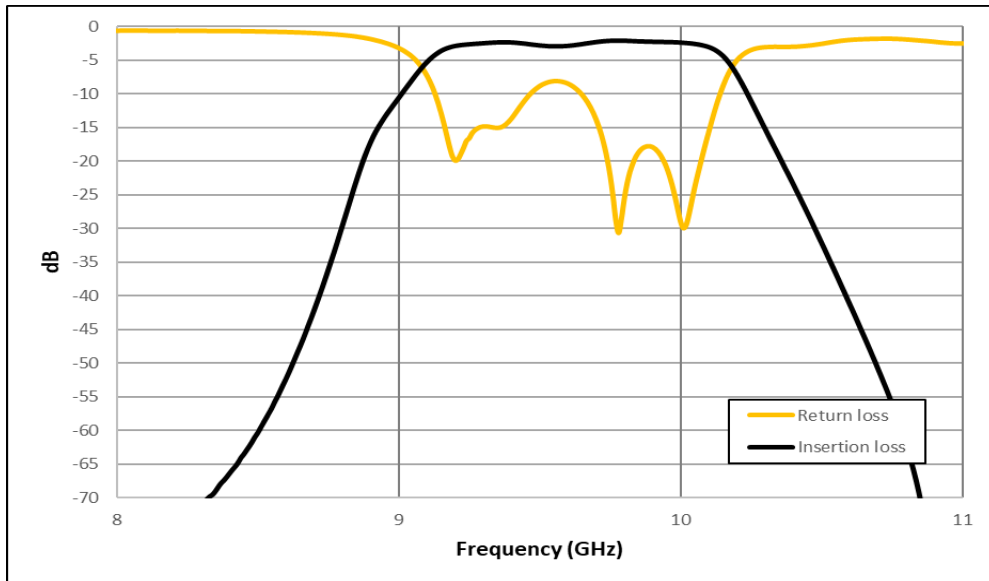
Figure 1: ERZ-BPF-0920-1000-2.9 Insertion & Return loss
