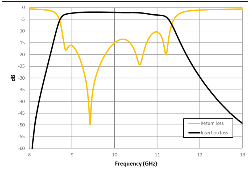
Figure 1: ERZ-BPF-0900-1100-3 Insertion & Return loss
