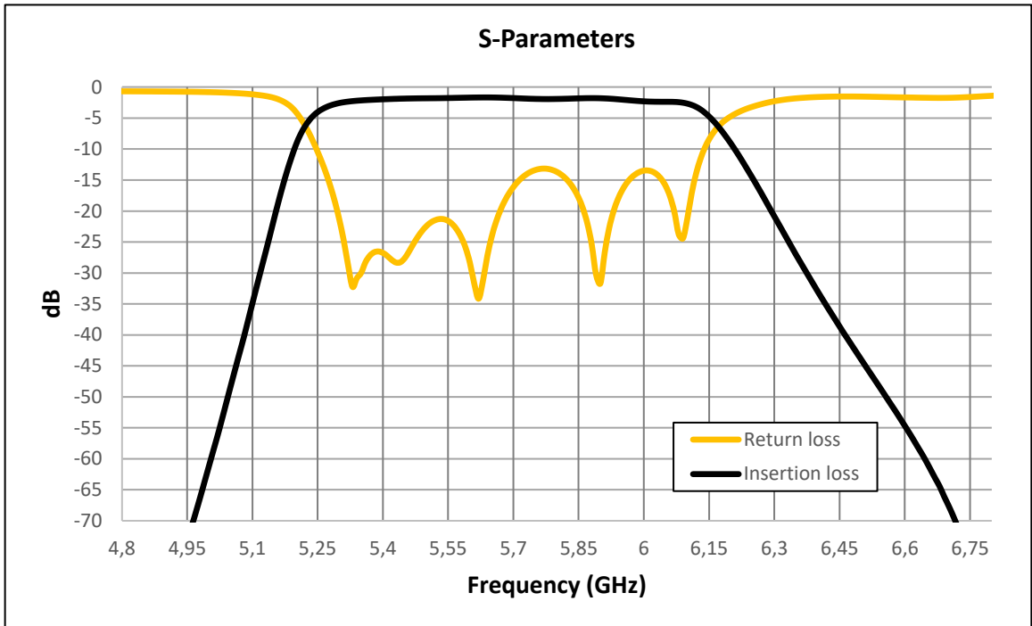
Figure 1:ERZ-BPF-0530-0610-2.5 Insertion & Return loss
