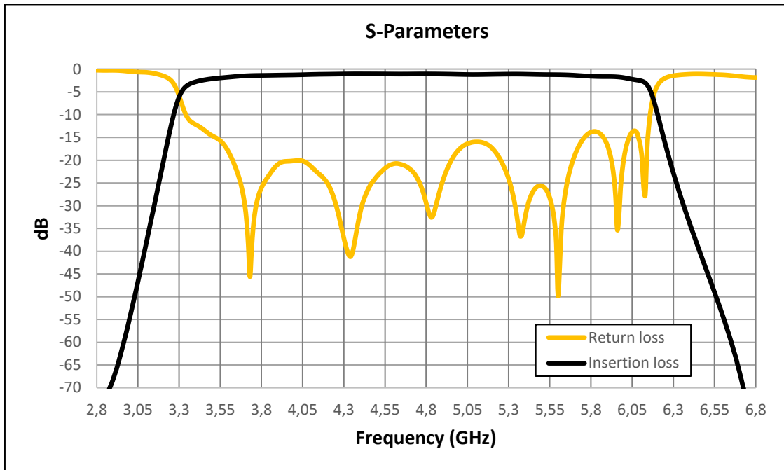
Figure 1:ERZ-BPF-0350-0610-2.1 Insertion & Return loss
