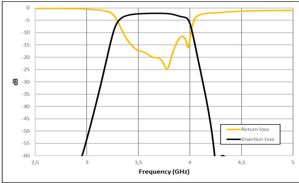
Figure 1: ERZ-BPF-0350-0380-2.4 Insertion & Return loss
