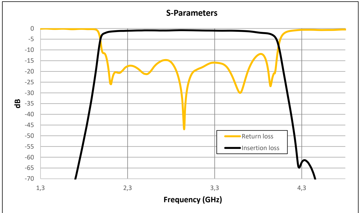
Figure 1:ERZ-BPF-0210-0380-1.9 Insertion & Return loss
