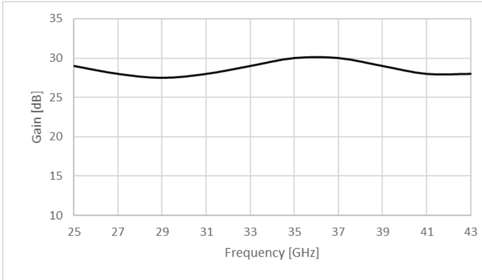
Figure 1: ERZ-LNA-2500-4300-33-2 Small Signal Gain
