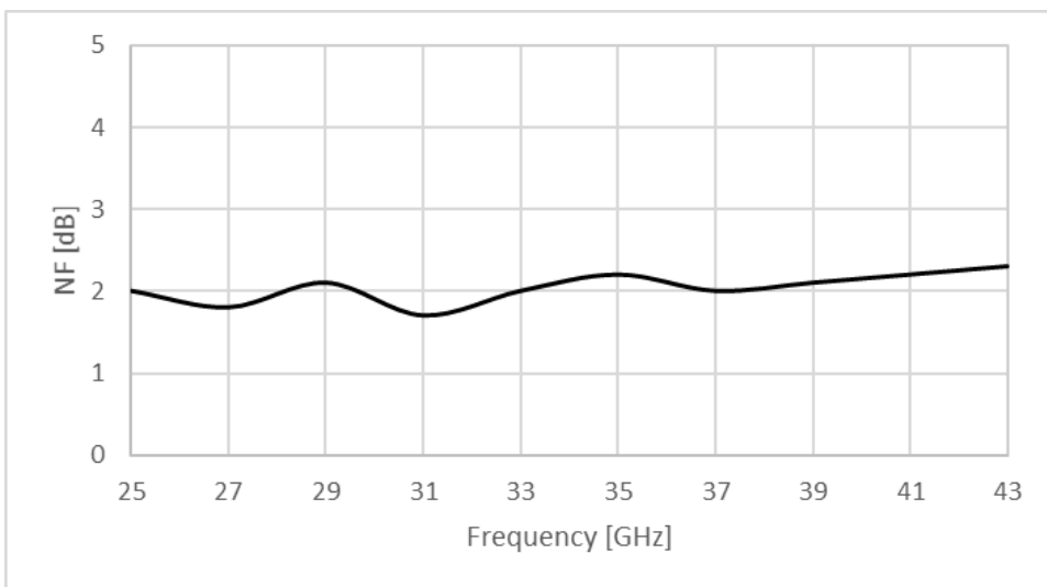
Figure 2: ERZ-LNA-2500-4300-33-2 Noise Figure
