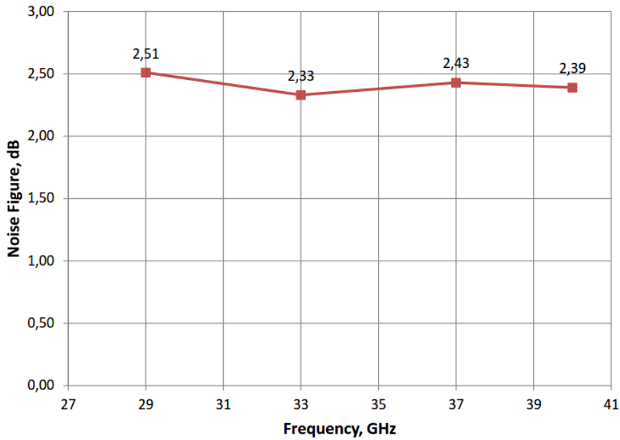
Figure 1-3: ERZ-LNA-2900-4000-30-2.5 Noise Figure
