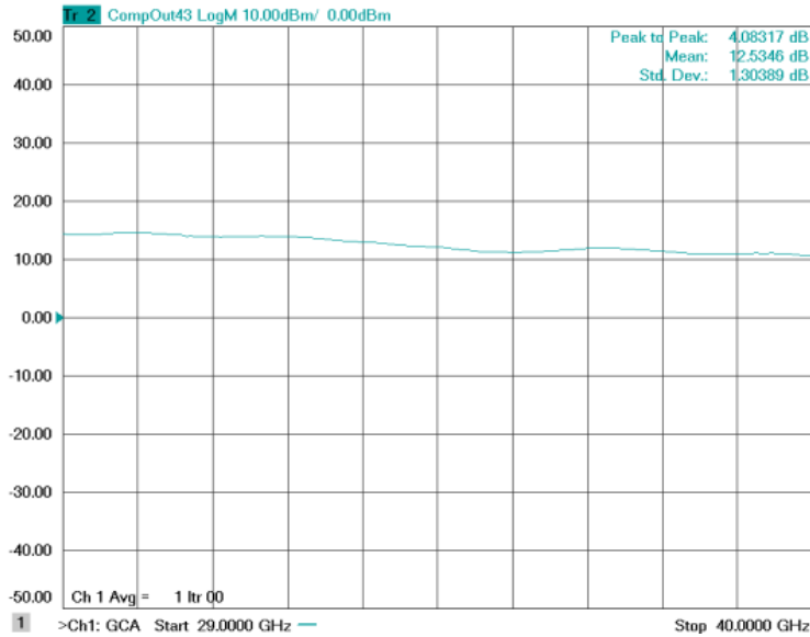
Figure 1-1: ERZ-LNA-2900-4000-30-2.5 P1dB
