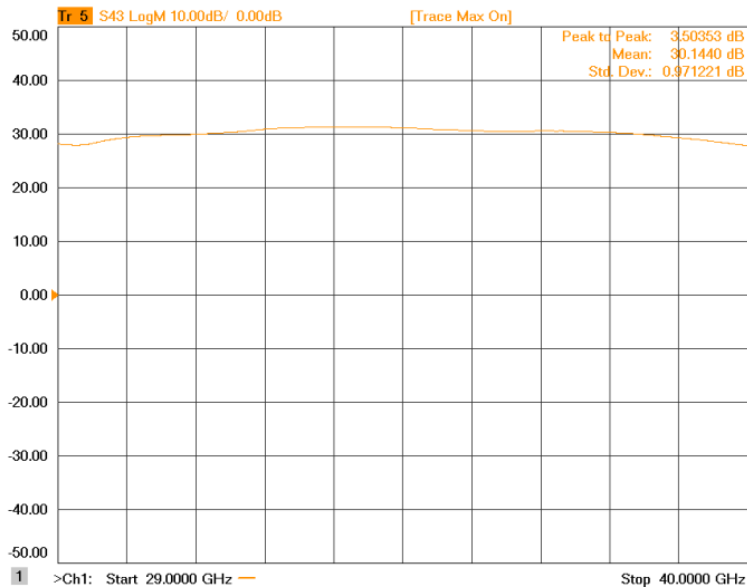
Figure 1-2: ERZ-LNA-2900-4000-30-2.5 Small Signal Gain
