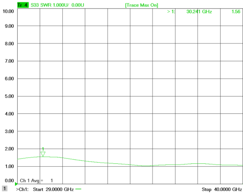
Figure 1-4: ERZ-LNA-2900-4000-30-2.5 Input Matching
