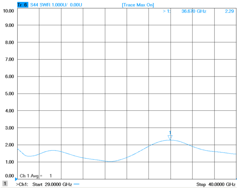
Figure 1-5: ERZ-LNA-2900-4000-30-2.5 Output Matching
