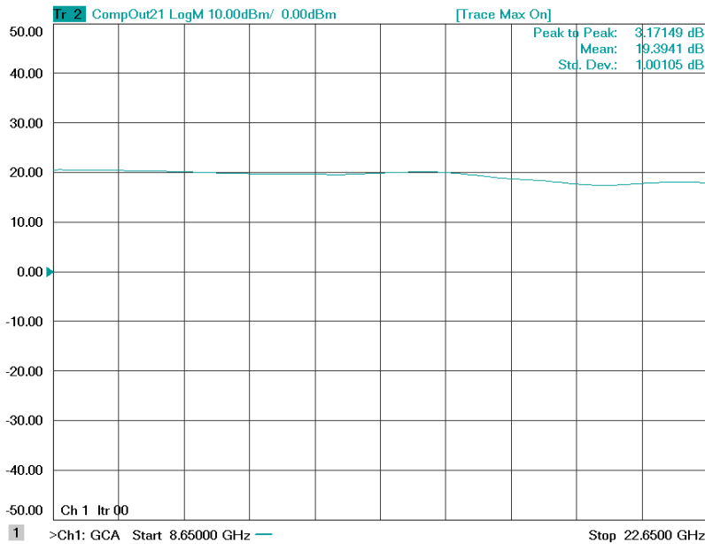
Figure 1: ERZ-LNA-0865-2265-30-3 P1dB
