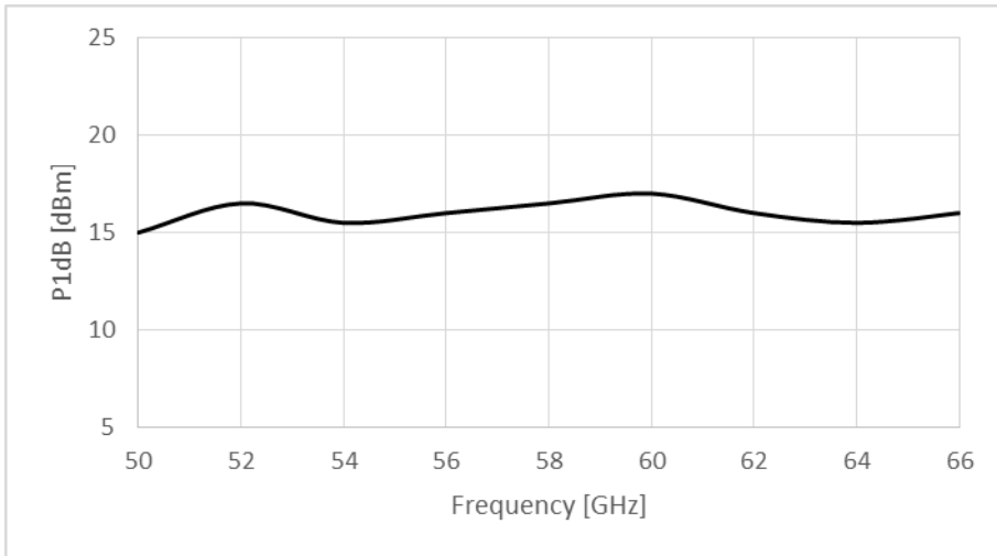
Figure 1: ERZ-HPA-5000-6600-19 P1dB
