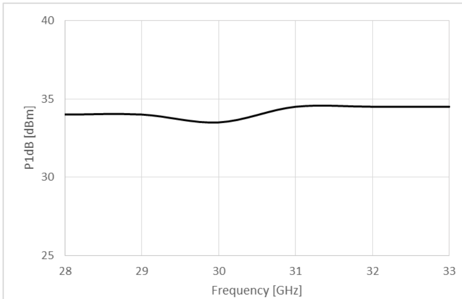
Figure 1: ERZ-HPA-2800-3300-33 P1dB
