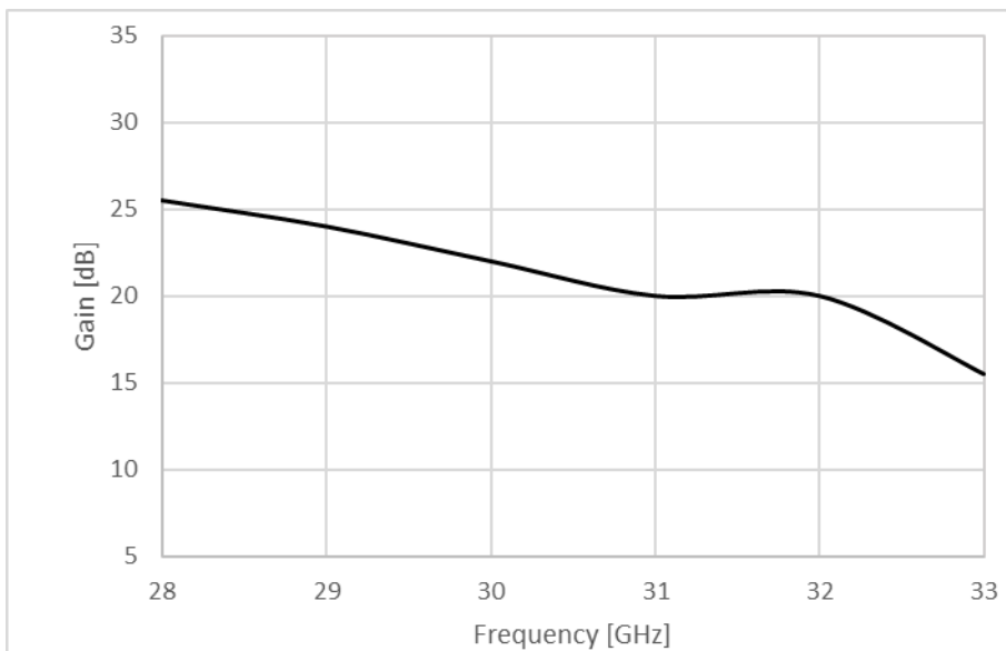
Figure 2: ERZ-HPA-2800-3300-33 Small Signal Gain
