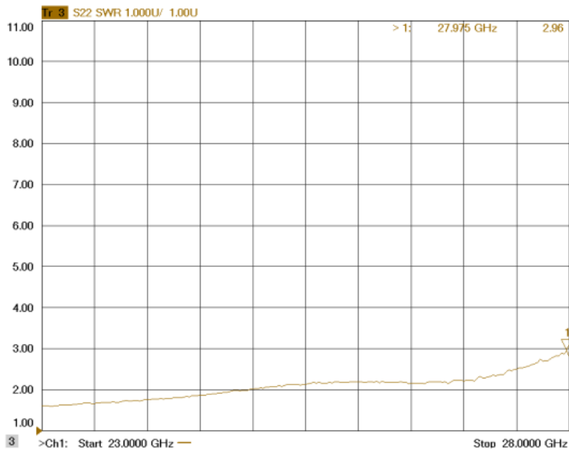
Figure 1-5: ERZ-HPA-2300-2800-32 Output Matching
