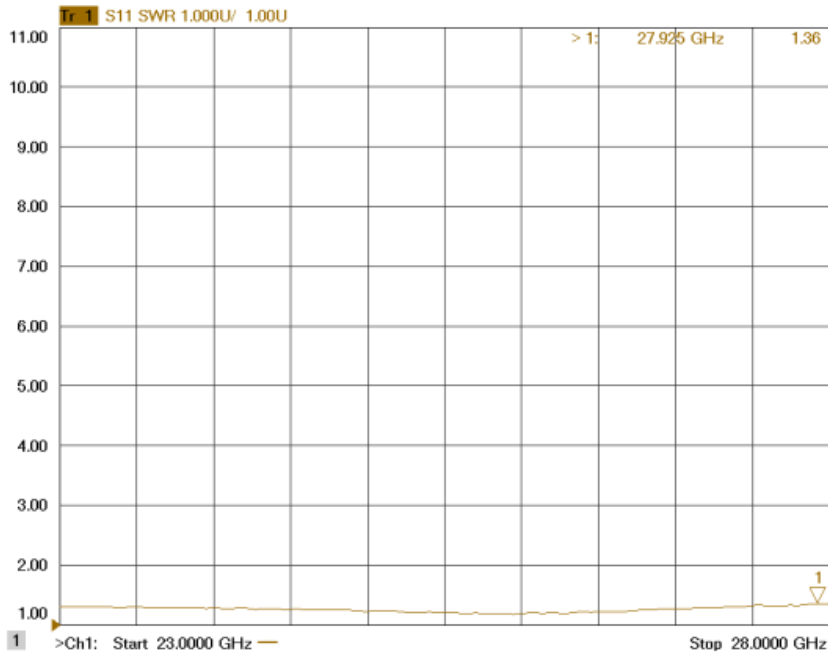
Figure 1-4: ERZ-HPA-2300-2800-32 Input Matching
