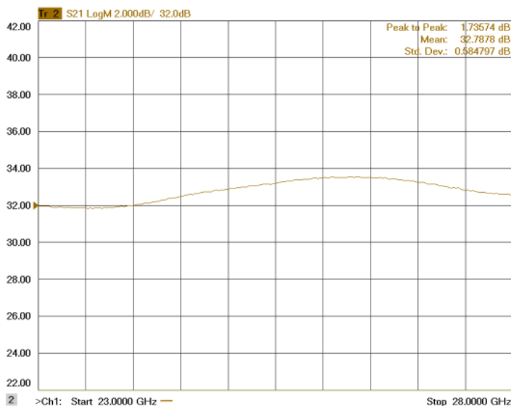
Figure 1-2: ERZ-HPA-2300-2800-32 Small Signal Gain
