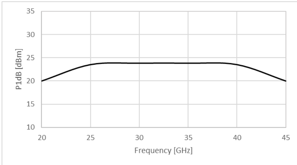
Figure 1: ERZ-HPA-2000-4500-24 P1dB
