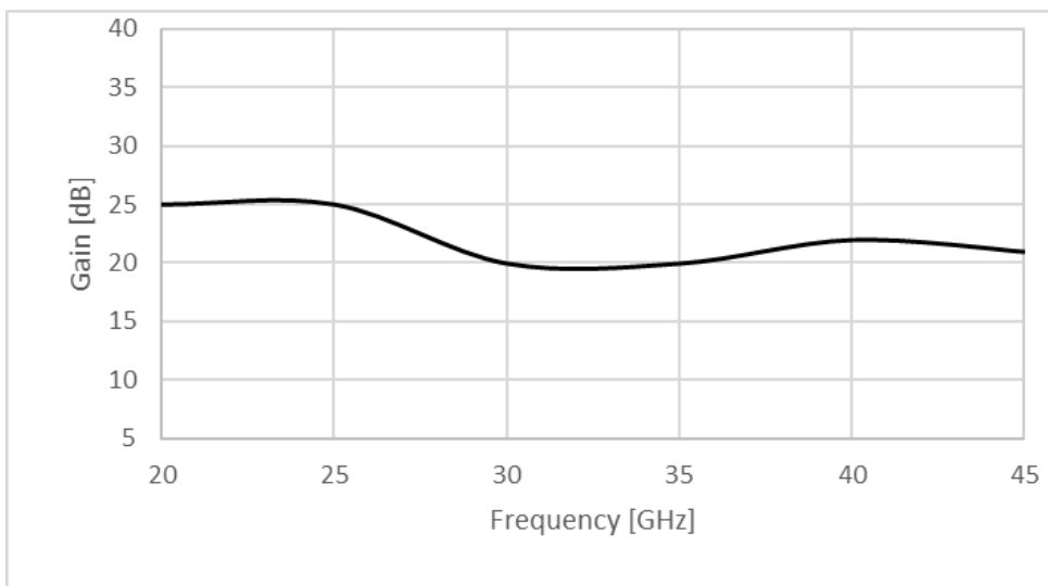
Figure 2: ERZ-HPA-2000-4500-24 Small Signal Gain
