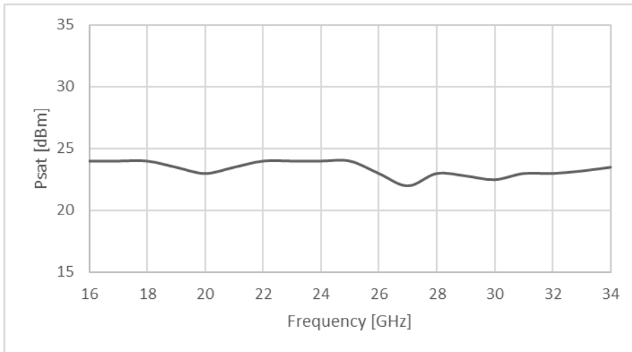
Figure 1: ERZ-HPA-1600-3300-24-E Psat
