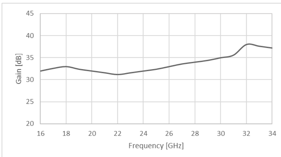
Figure 2: ERZ-HPA-1600-3300-24-E Small Signal Gain
